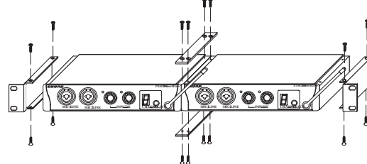
Dual-Mounting Two Units
