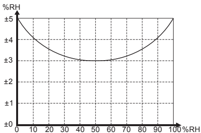
Fig. (19) Relative Humidity Accuracy
