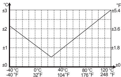
Fig. (20) Temperature Accuracy
