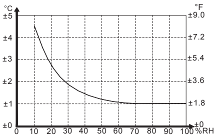
Fig. (21) Dew Point Accuracy (at 25°C)
