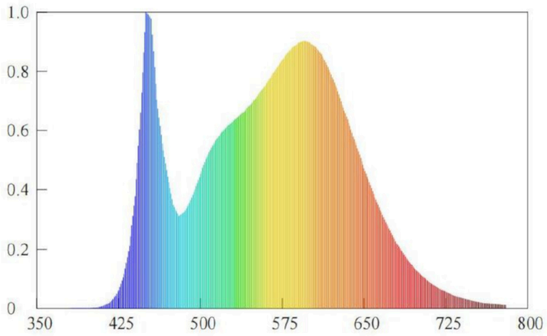
Spectral power distribution(24W 4000K)
